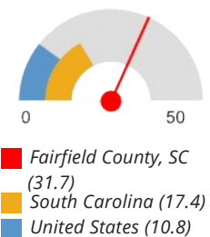
Motor Vehicle Accident Mortality, Age Adj. Rate (Per 100,000 Pop.) by County, NVSS 2009-13
